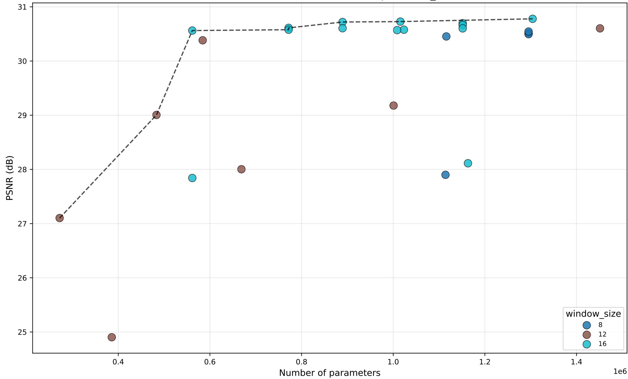
PSNR vs #Params — OmniSR — by window_size
